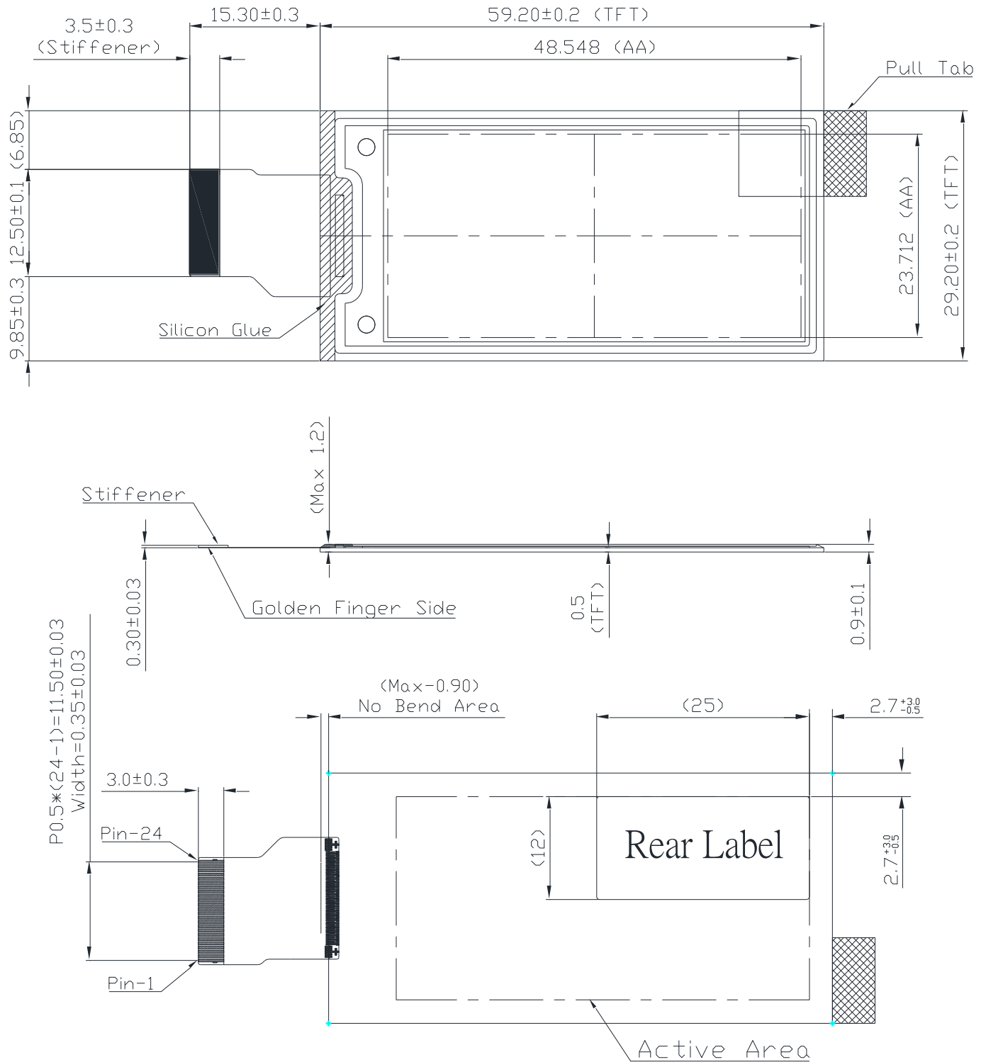
Figure 1-1 EPD Drawing
