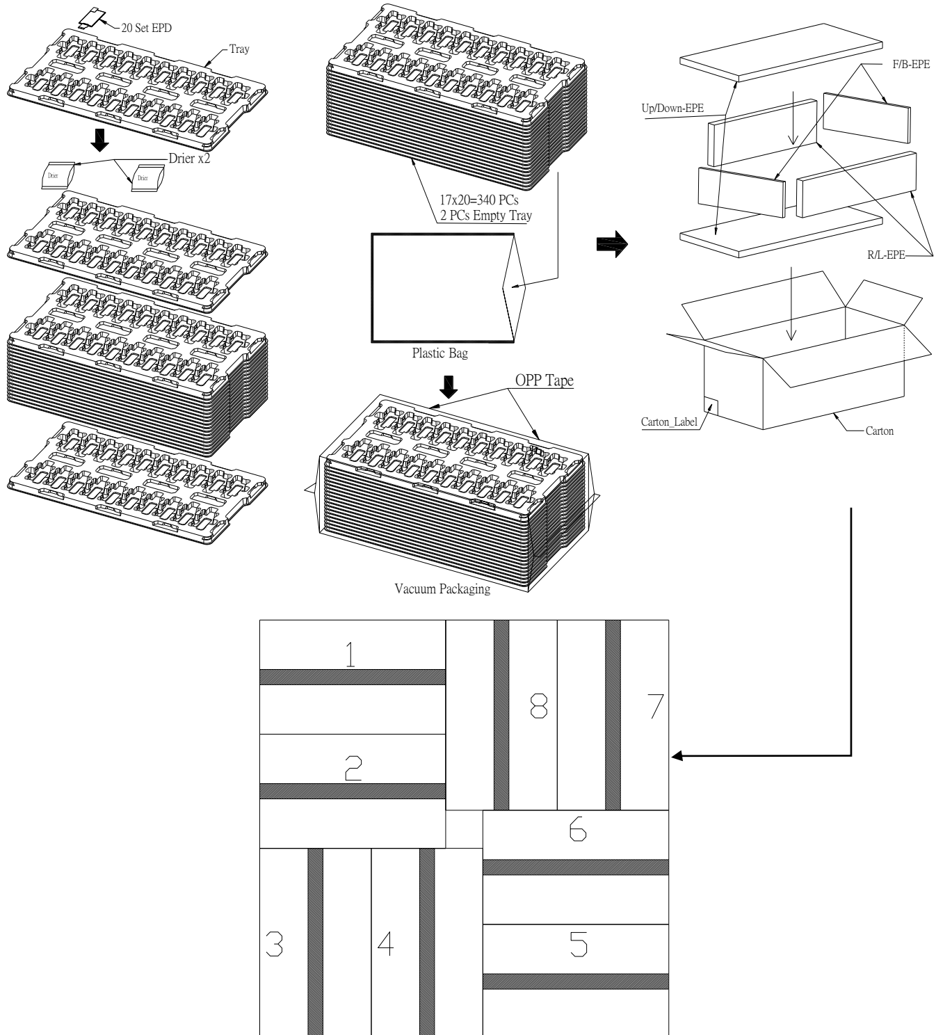
Figure 7-1 Packing Diagram
